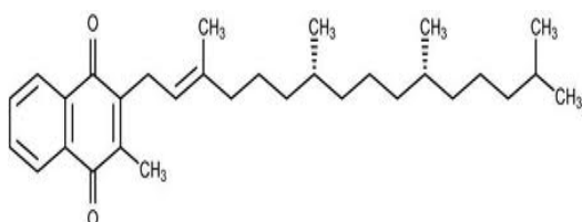
Figure 1. Chemical structure of trans -vitamin K 1 .
